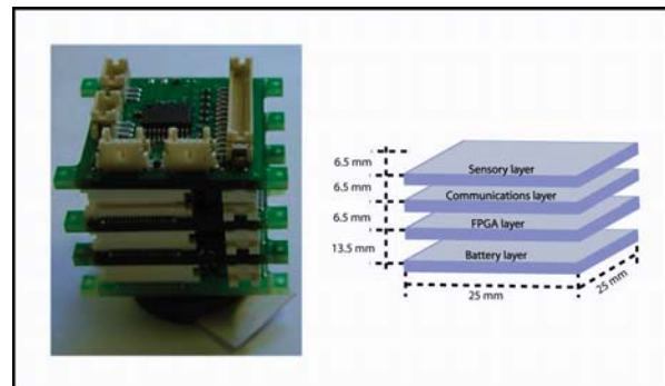
Figure 4 - 25mm 3 Core
