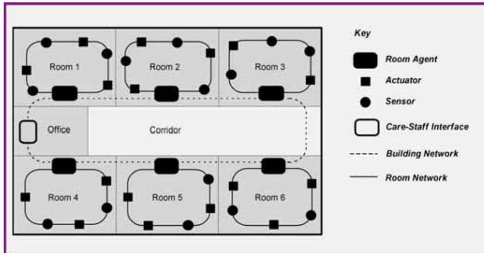
Figure 1. The Decentralised Architecture
