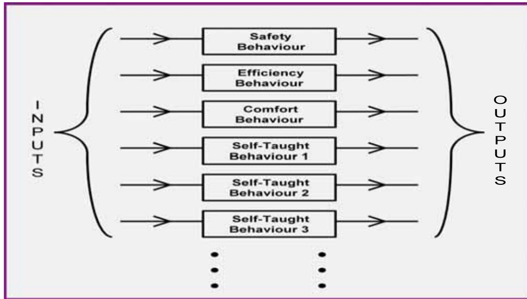
Figure 2. Overview of the agent architecture
