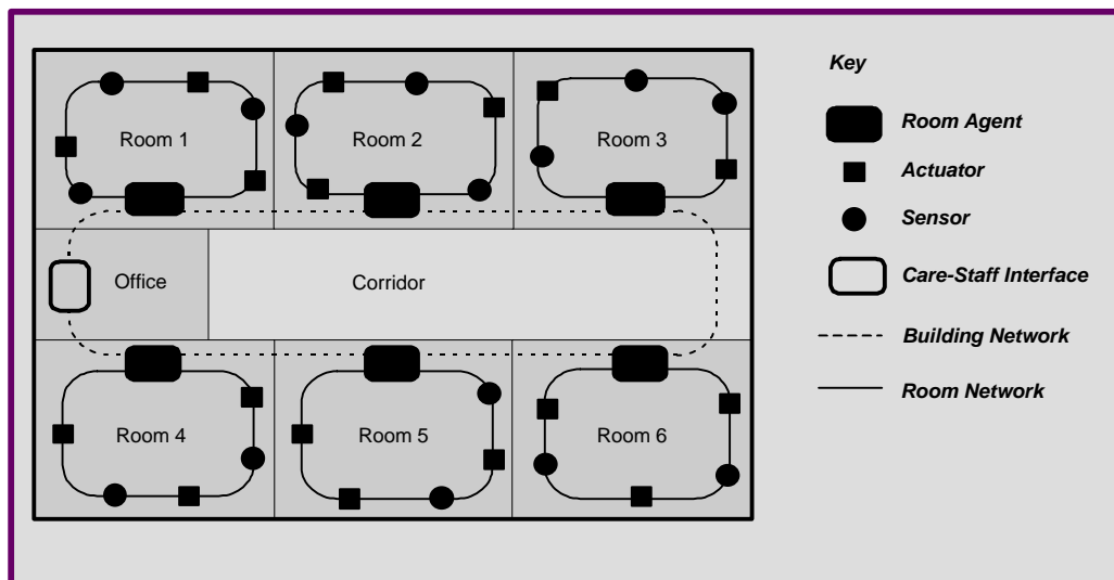
The Decentralised Architecture
